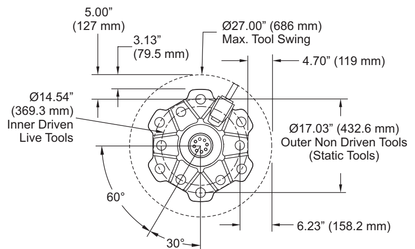
12-Station VDI Turret Option
