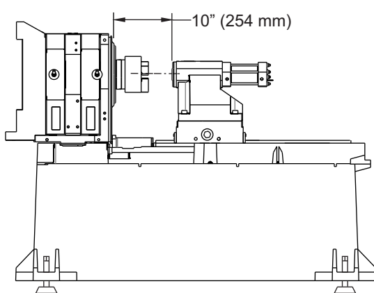
ST-10 Tailstock Travel #3 Morse Taper
