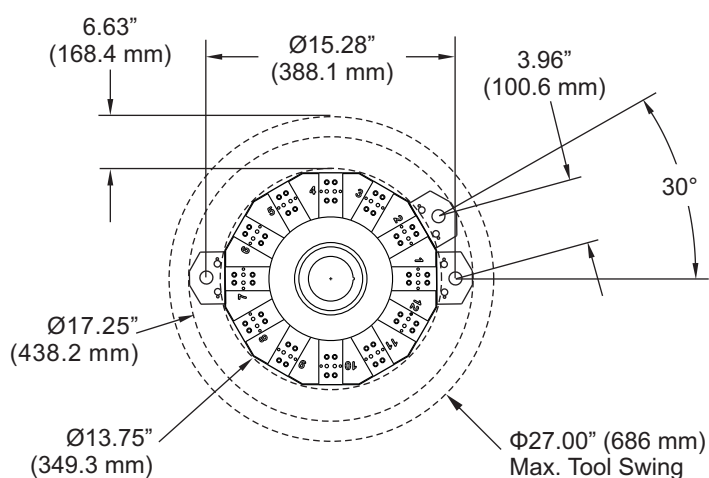
12-Station BOT Turret Standard
