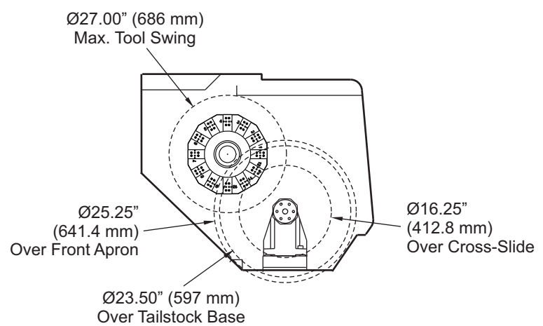
ST-10 Tool Swing Envelope Turret at Home Position 12-Station BOT Turret Standard VDI Turret Standard (HAE only)
