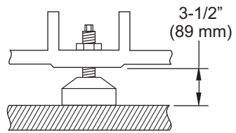
4X Leveling Pad Pin Dimension
